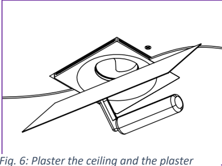
Fig. 6: Plaster the ceiling and the plaster fitting.
