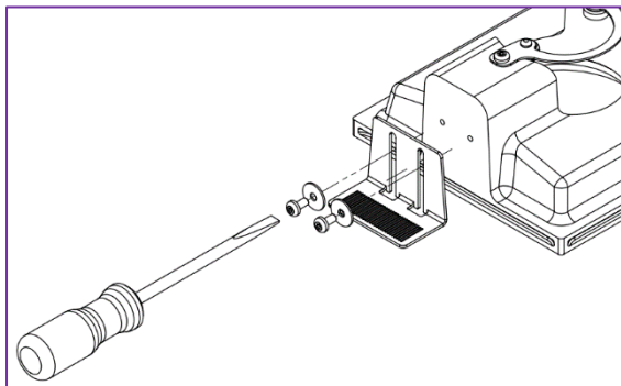
Fig. 3: Set the correct height of the mounting angles.
