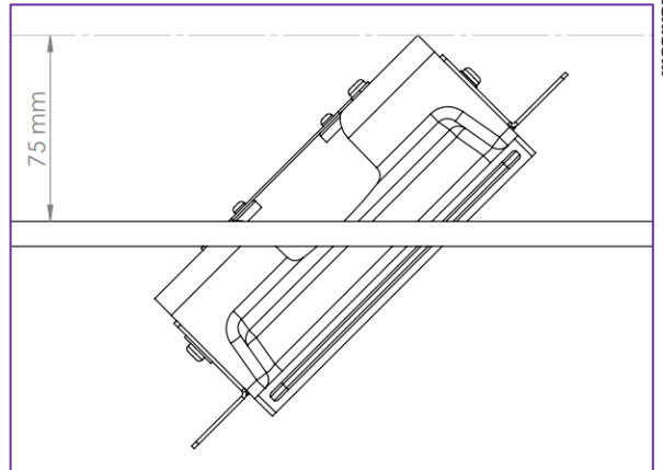
Fig. 2: Bring the Plaster fixing at an angle in position. Minimum height of 75 mm is required
