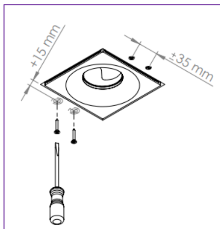
Fig. 4: Screw the fixing onto the ceiling
