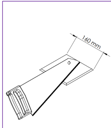
Fig. 1 Saw the hole 160x160 mm
